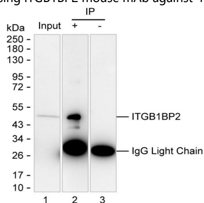
Western blot analysis using ITGB1BP2 mouse mAb against rat skeletal muscle lysate
