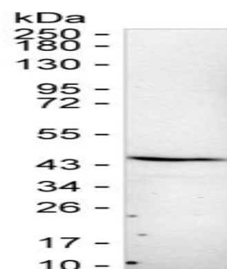
Western blot analysis using ITGB1BP2 mouse mAb against rat skeletal muscle lysate
