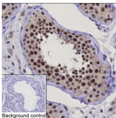
IHC-P analysis of testis tissue by FKBP5 antibody (AMM83212)
