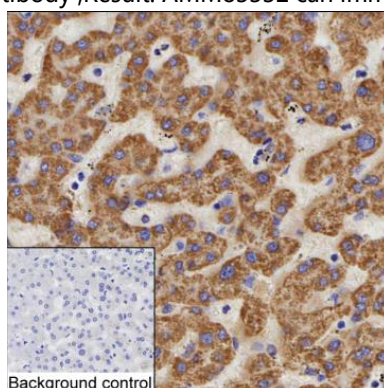
IHC-P analysis of liver tissue by DECR1 antibody (AMM83332)
