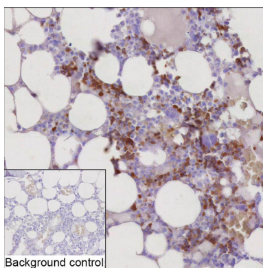
IHC-P analysis of bone marrow tissue by DEFA1 antibody (AMM83432)
