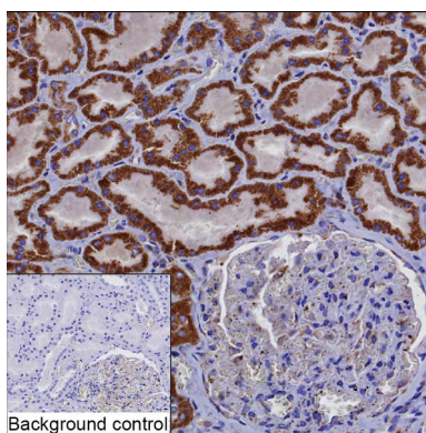
IHC-P analysis of kidney tissue by ATP6AP2 antibody (AMM83494)
