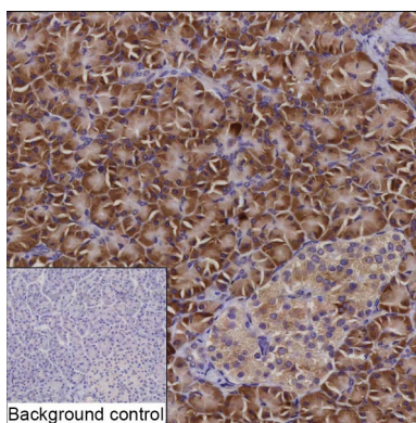
IHC-P analysis of pancreas tissue by MANF antibody (AMM83515)
