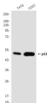
Western blot analysis of p53 in T47D and COS7 lysates using p53 antibody
