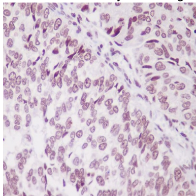
Immunohistochemistry analysis of paraffin-embedded Human bladder cancer using PARK7 antibody. High-pressure and temperature Sodium Citrate pH 6.0 was used for antigen retrieval.
