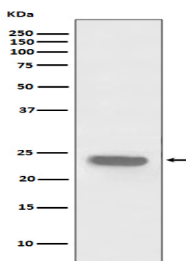
Western blot analysis of PARK7 in HeLa lysates using PARK7/DJ1 antibody.
