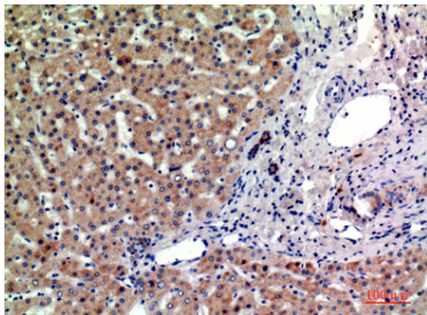
Immunohistochemistry analysis of paraffin-embedded Human liver using CD315 antibody. High-pressure and temperature Sodium Citrate pH 6.0 was used for antigen retrieval.
