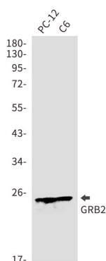
Western blot analysis of GRB2 in PC-12, C6 lysates using GRB2 antibody.
