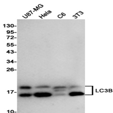
Western blot analysis of LC3B in U87-MG, HeLa, C6 and 3T3 lysates using LC3B antibody.
