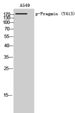
Western Blot analysis of A549 cells using Phospho-Pragmin (Y413) Polyclonal Antibody
