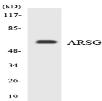
Western blot analysis of the lysates from HeLa cells using ARSG antibody.
