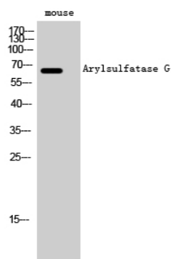
Western Blot analysis of mouse cells using Arylsulfatase G Polyclonal Antibody
