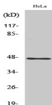
Western Blot analysis of various cells using AW-1 Polyclonal Antibody
