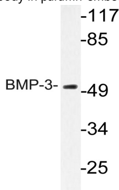
Western blot analysis of lysate from HeLa cells, using BMP-3 antibody.
