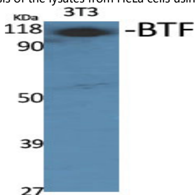
Western Blot analysis of various cells using BTF Polyclonal Antibody
