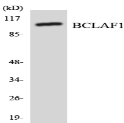
Western blot analysis of the lysates from HeLa cells using BCLAF1 antibody.
