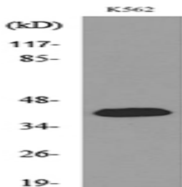
Western blot analysis of lysate from K562 cells, using CX3CL1 Antibody.
