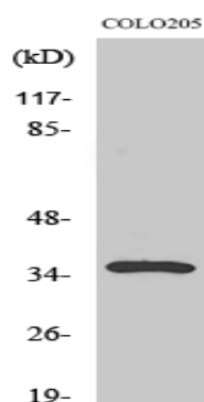
Western Blot analysis of various cells using Galectin-4 Polyclonal Antibody
