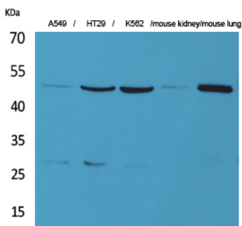
Western Blot analysis of A549, HT29, K562, mouse kidney, mouse lung cells using GDI-2 Polyclonal Antibody.. Secondary antibody was diluted at 1:20000
