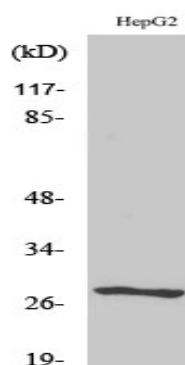
Western Blot analysis of various cells using NPDC-1 Polyclonal Antibody
