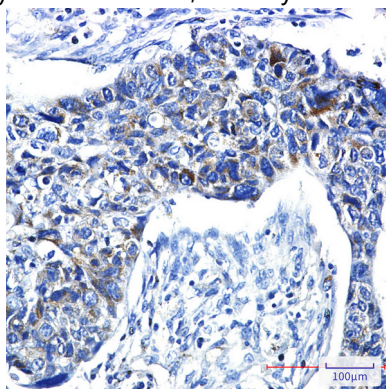
Immunohistochemistry analysis of paraffin-embedded Human lung cancer using PRC1 antibody. High-pressure and temperature Sodium Citrate pH 6.0 was used for antigen retrieval.
