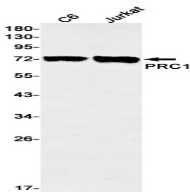
Western blot analysis of PRC1 in C6, Jurkat lysates using PRC1 antibody.
