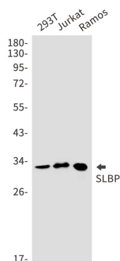
Western blot analysis of SLBP in 293T, Jurkat, Ramos lysates using SLBP antibody.
