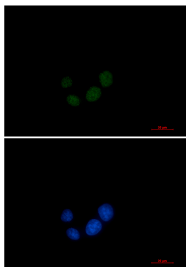
Immunocytochemistry analysis of SPT5 (green) in HeLa using SPT5 antibody, and DAPI (blue).
