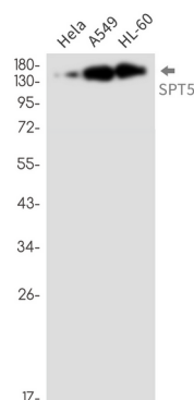
Western blot analysis of SPT5 in HeLa, A549, HL-60 lysates using SPT5 antibody.
