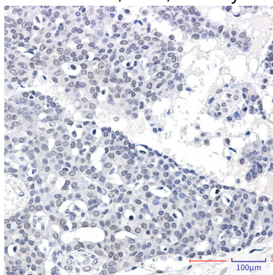
Immunohistochemistry analysis of paraffin-embedded Human breast cancer tissue using SPT5 antibody. High-pressure and temperature Sodium Citrate pH 6.0 was used for antigen retrieval.
