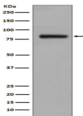
Western blot analysis of GOLPH2 expression in LnCaP cell lysate.
