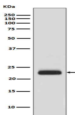
Western blot analysis of RAIDD expression in HeLa cell lysate.
