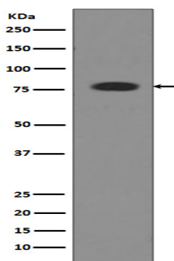
Western blot analysis of Transferrin expression in Human serum lysate.
