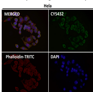
Immunofluorescent analysis using the Antibody at 1:200 dilution.
