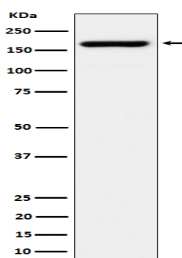
Western blot analysis of eIF3A expression in Jurkat cell lysate.
