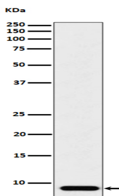
Western blot analysis of ATP5G1 expression in HeLa cell lysate.
