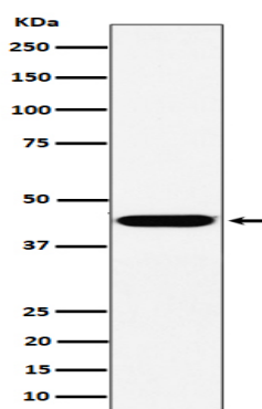
Western blot analysis of KCTD9 expression in HepG2 cell lysate.
