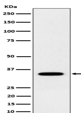
Western blot analysis of NTH1 expression in 293 cell lysate.
