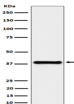
Western blot analysis of UCHL5IP expression in HeLa cell lysate.
