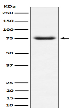
Western blot analysis of PWP1 expression in HepG2 cell lysate.
