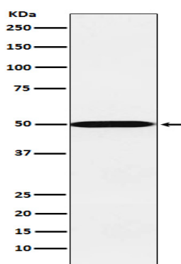
Western blot analysis of CYP26A1 expression in HepG2 cell lysate.
