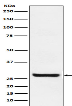
Western blot analysis of Sprouty 4 expression in MCF7 cell lysate.
