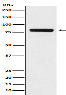
Western blot analysis of SEC23 expression in HeLa cell lysate.
