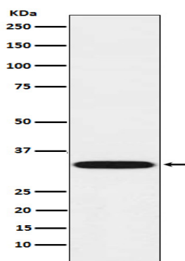
Western blot analysis of TREX1 expression in Daudi cell lysate.
