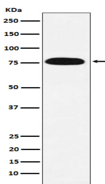
Western blot analysis of KHSRP expression in HeLa cell lysate.
