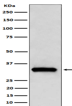
Western blot analysis of NDUFAF1 expression in 293T cell lysate.
