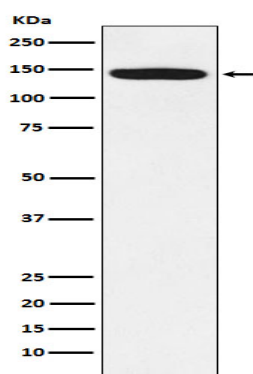
Western blot analysis of HTSF1 expression in Jurkat cell lysate.
