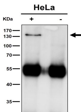
Immunoprecipitate (IP) analysis using the Antibody at 1:50 dilution. (wb at 1:3K dilution)
