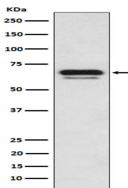
Western blot analysis of p66 alpha expression in K562 cell lysate.
