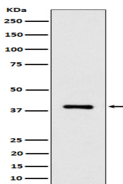
Western blot analysis of ACAT2 expression in K562 cell lysate.
