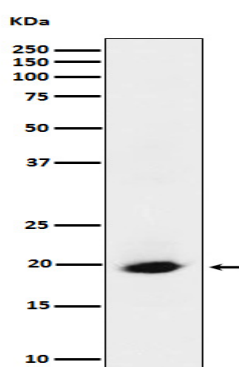
Western blot analysis of SRP19 expression in HeLa cell lysate.
