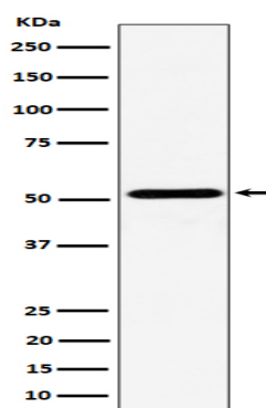
Western blot analysis of NPY5R expression in Ramos cell lysate.
