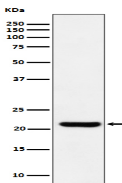
Western blot analysis of ITPA expression in HepG2 cell lysate.
