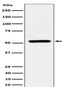
Western blot analysis of ADRA1A expression in HepG2 cell lysate.
