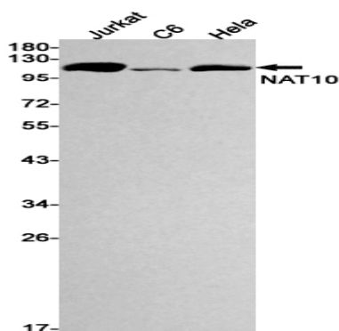
Western blot analysis of NAT10 in Jurkat, C6, HeLa lysates using NAT10 antibody.
