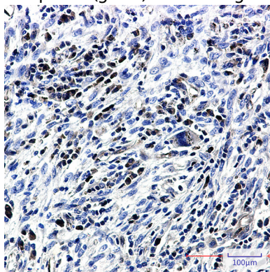
Immunohistochemistry analysis of paraffin-embedded Human lung cancer tissue using Caspase3 antibody. High-pressure
