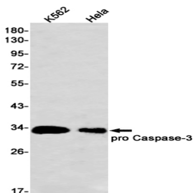
Western blot analysis of Caspase3 in K562, HeLa lysates using Caspase3 antibody.
