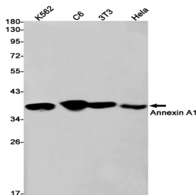
Western blot analysis of Annexin A1 in K562, C6, 3T3, HeLa lysates using Annexin A1 antibody.
