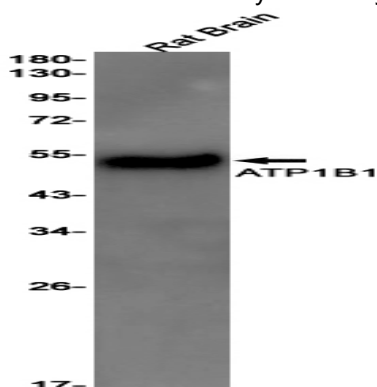
Western blot analysis of ATP1B1 in rat Brain lysates using ATP1B1 antibody.
