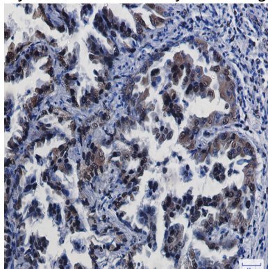
Immunohistochemistry analysis of paraffin-embedded Human lung cancer using CREB antibody. High-pressure and temperature Sodium Citrate pH 6.0 was used for antigen retrieval.
