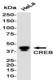
Western blot analysis of CREB in 3T3 lysates using CREB antibody.
